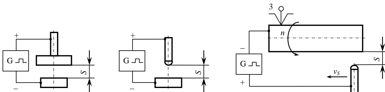
Fig. 1. Technological schemes of the oxide pellicle formation by applying EDI:
